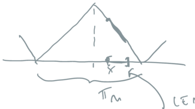
Figure 3.6: Demonstration of monotonicity
