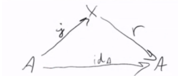
Figure 6.11: The retraction r gives a left inverse to the map induced by inclusion.
