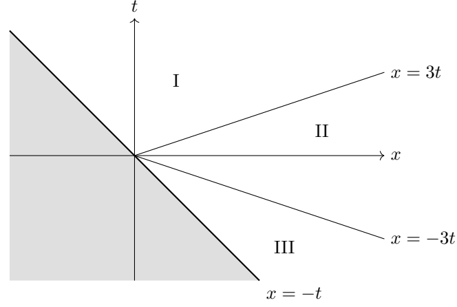
Figure 2.2: The regions of example 2.2.1: u = -\cos(x + 3t) - 2\cos(\frac{x-3t}{2}) + 7 in I, u = -\cos(x + 3t) + 5\cos(x - 3t) in II, and u = \frac{5}{2}\cos(2x + 6t) - \frac{7}{2} + 5\cos(x - 3t) in III. The shaded half-plane x < -t lies outside the domain
