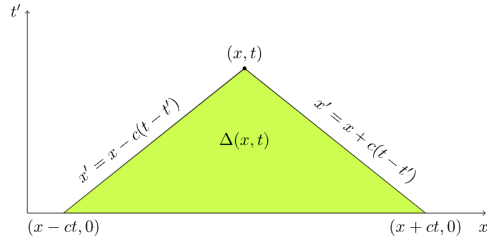
Figure 2.1: The backwards light cone of (t, x) and the triangle \Delta(x, t) it encloses, drawn for propagation speed c , which is 1 here
