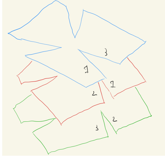
Figure 5.2: 3 sheets with numbers represent which sheet to go to after crossing
