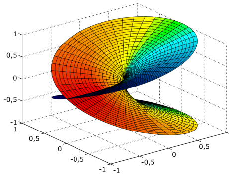
Figure 5.1: Branch Covering for \sqrt{\cdot}
