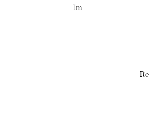
Figure 1.1: Complex Plane
