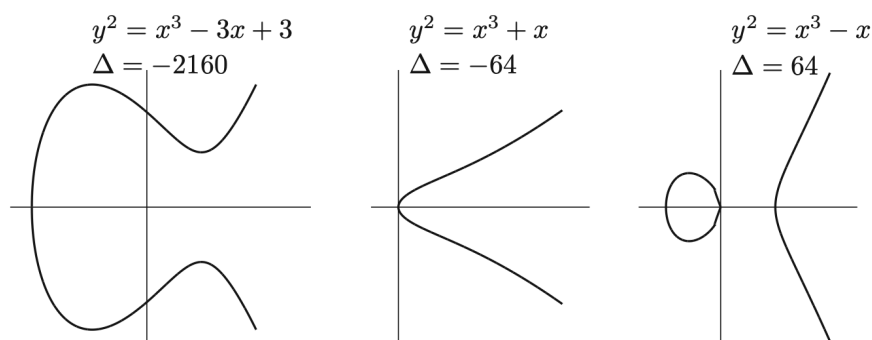
Figure 1.1: Silverman: Three Elliptic Curves
