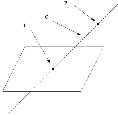
Figure 2.6: Codimension Pathology
