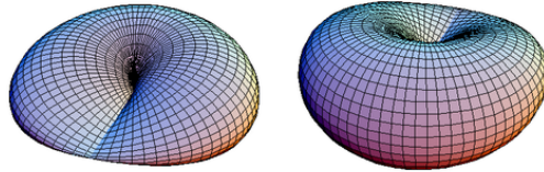
Figure 21.2: Wikipedia: Immersion of \mathbb{RP}^2
