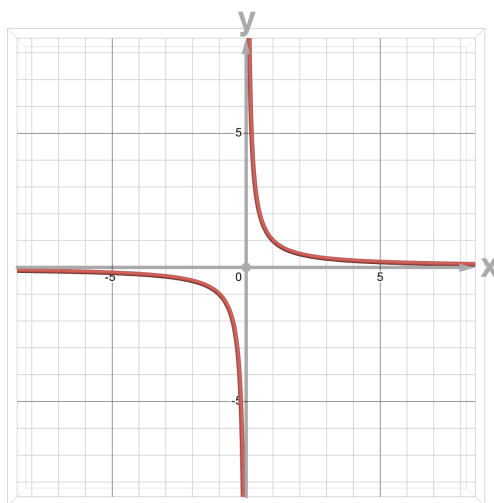
Figure 28.4: zero-set of xy = 1
