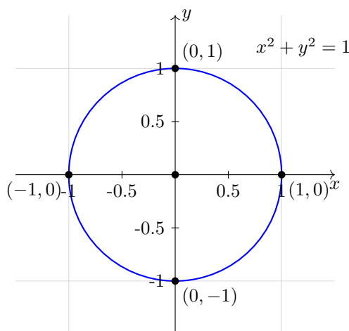
Figure 28.1: Circle represented by the equation x^2 + y^2 - 1 = 0
