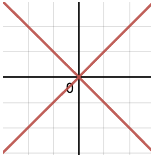
Figure 22.3: Approximate Geometric picture corresponding to \varprojlim R/(x, y)^n
