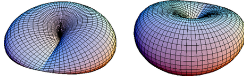
Figure 28.2: Wikipedia: Immersion of \mathbb{RP}^2
