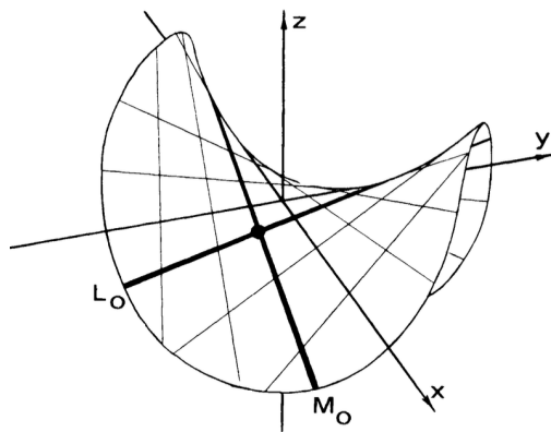
Figure 28.8: Serge Embedding of Product of Projective Lines
