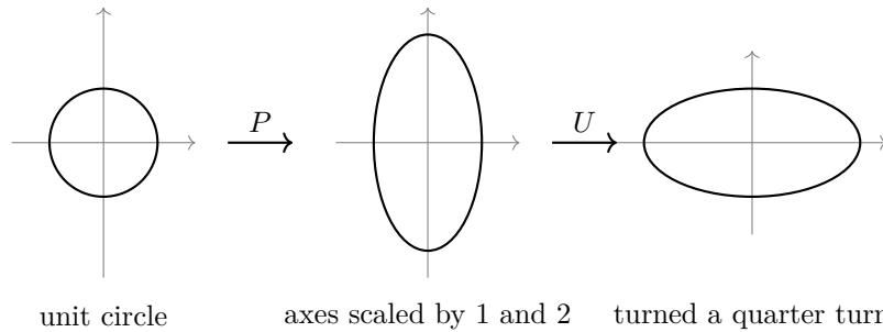
Figure 11.3: The image of the unit circle under the two factors of A = UP
