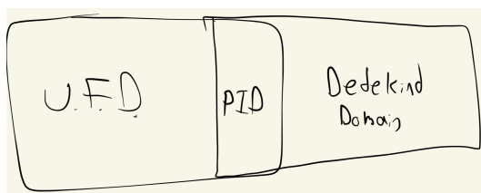
Figure 45.1: Venn diagram
