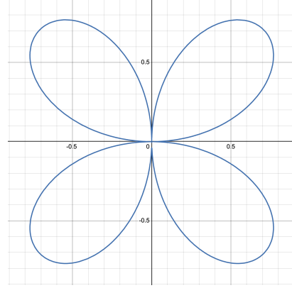
Figure 38.2: Four-Leaf Curve
