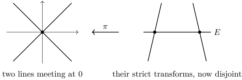
Figure 15.1: Blowing up separates the branches of a node. The exceptional divisor E records the direction along which each branch approaches the origin.
