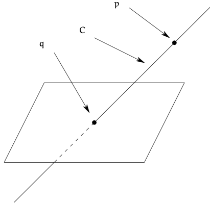
Figure 2.7: Codimension Pathology
