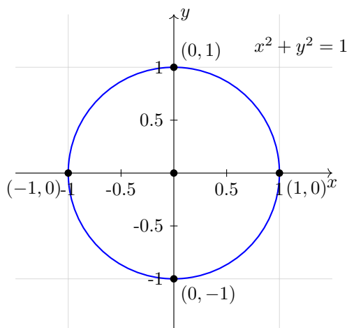
Figure 1.1: Circle represented by the equation x^2 + y^2 - 1 \in \mathbb{R}[x, y]
