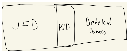
Figure 50.1: Venn diagram
