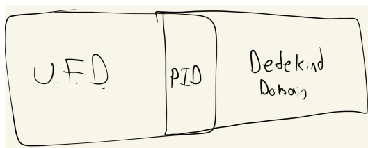
Figure 50.1: Venn diagram
