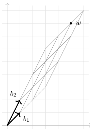
Figure 2.9: Lines parallel to b_1 and b_2 through the integer combinations of b_1 and b_2 form a grid, and w = 2b_1 + 3b_2 is two steps along b_1 and three along b_2
