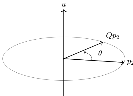
Figure 7.6: A matrix of \text{SO}(3) fixes the line \mathbb{R}u and turns the plane (\mathbb{R}u)^\perp through \theta
