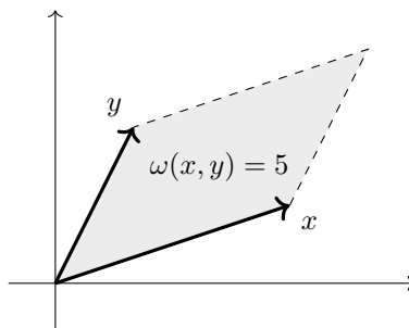
Figure 10.1: The value of the symplectic form on \mathbb{R}^2 at x = (3, 1)^\top and y = (1, 2)^\top is the signed area 3 \cdot 2 - 1 \cdot 1 of the parallelogram they span
