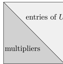
Figure 1.7: For a square matrix the two factors fit in one array: elimination leaves U on and above the diagonal, and the multiplier used to clear position (i, j) can be stored in that position
