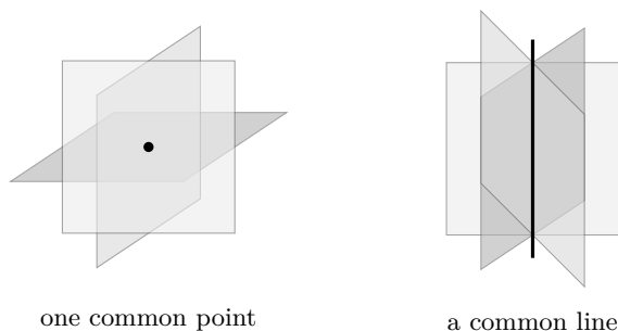
Figure 1.2: Three planes meeting in a single point, and three planes meeting in a line
