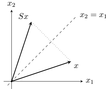
Figure 7.1: The operator S of example 7.1.2 exchanges the two coordinates, reflecting each vector across the line x_2 = x_1
