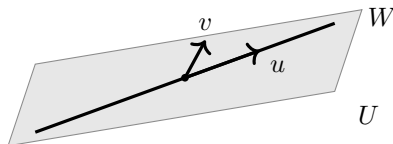
Figure 2.5: A line U = \text{span}\{u\} inside a plane W = \text{span}\{u, v\} in \mathbb{R}^3 , with \dim U = 1 and \dim W = 2
