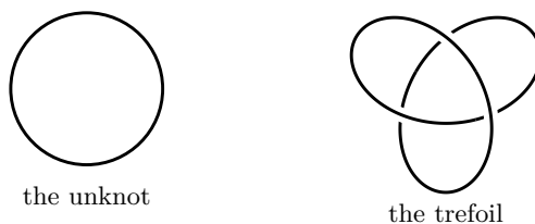
Figure 1: Two circles in \mathbb{R}^3 . They are homeomorphic, since each is a circle, but no motion of \mathbb{R}^3 carries one to the other. Homeomorphism compares the spaces themselves, not the way they sit in an ambient space.
