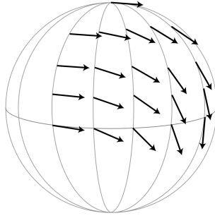
Figure 1.1: v_+ on D_+^2 (from Hatcher [14])
