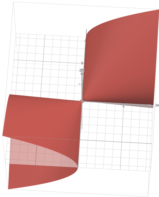
Figure 21.5: affine cone: xy - z^2
