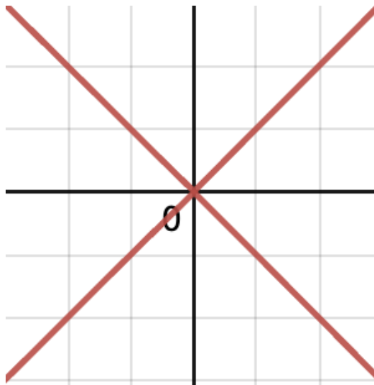
Figure 20.3: Approximate Geometric picture corresponding to \varprojlim R/(x, y)^n
