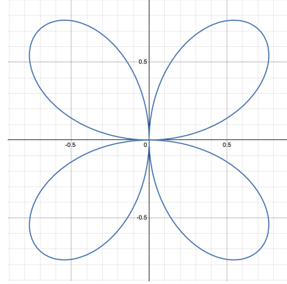
Figure 21.10: Four-Leaf Curve
