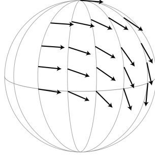
Figure 1.1: v_+ on D_+^2 (from Hatcher [11])
