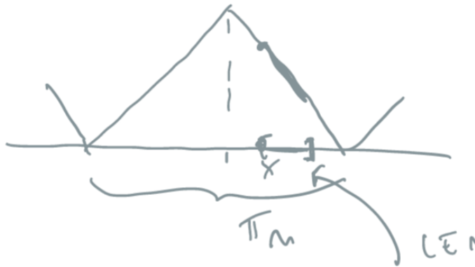
Figure 1.7: Demonstration of monotonicity
