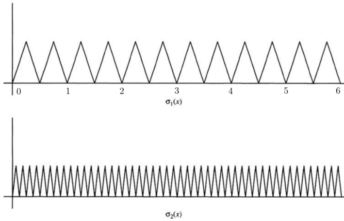
Figure 5.6: two examples of the iteration
