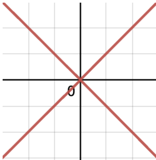
Figure 1.3: Approximate Geometric picture corresponding to \varprojlim R/(x, y)^n
