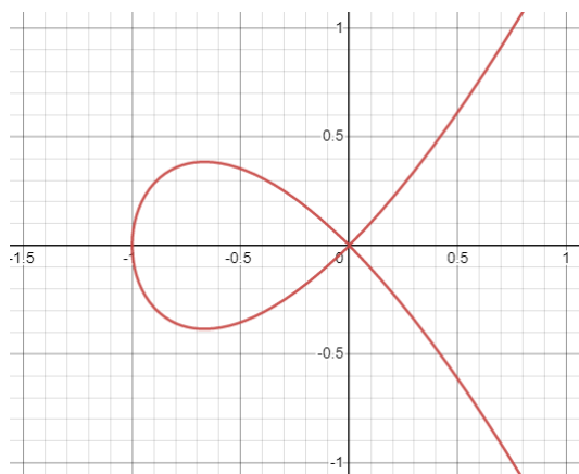
Figure 1.1: zero set of y^2 - x^2(x+1) = 0
