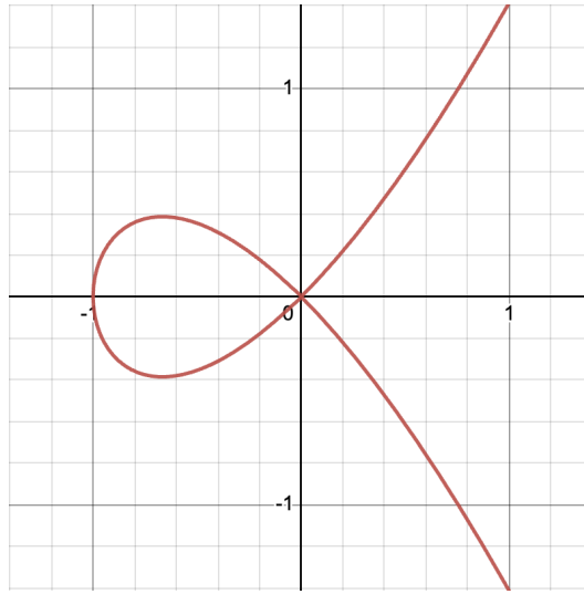
Figure 1.2: y^2 = x^3 + x^2
