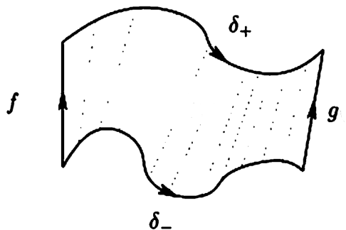
Figure 34.1: homotopy
