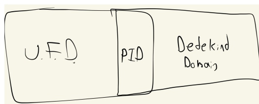
Figure 28.1: Venn diagram
