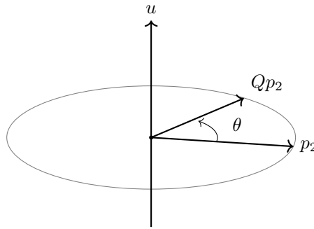
Figure 7.6: A matrix of SO(3) fixes the line \mathbb{R}u and turns the plane (\mathbb{R}u)^\perp through \theta
