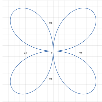
Figure 21.10: Four-Leaf Curve
