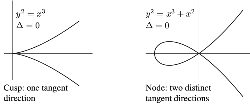
Figure 1.2: Silverman: singular Cubics
