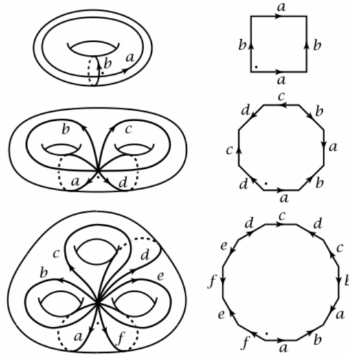
Figure 1.5: n -torus as CW complex, Hatcher
