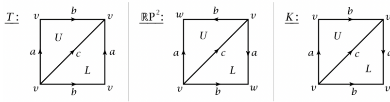
Figure 3.1: Different ways to glue a square
