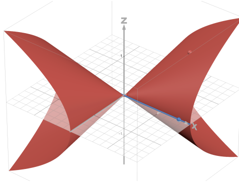
Figure 5.1: A ruling on the quadric cone
