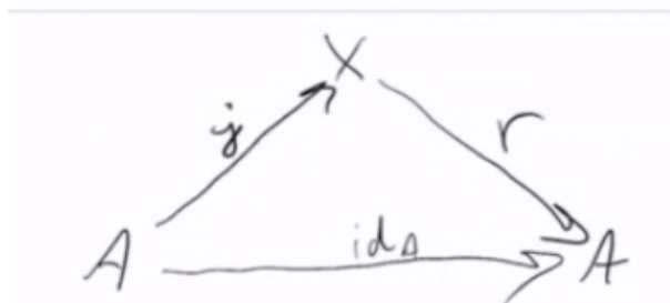
Figure 6.11: The retraction r gives a left inverse to the map induced by inclusion.
