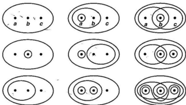
Figure 1.1: All topologies on a three-element set.
