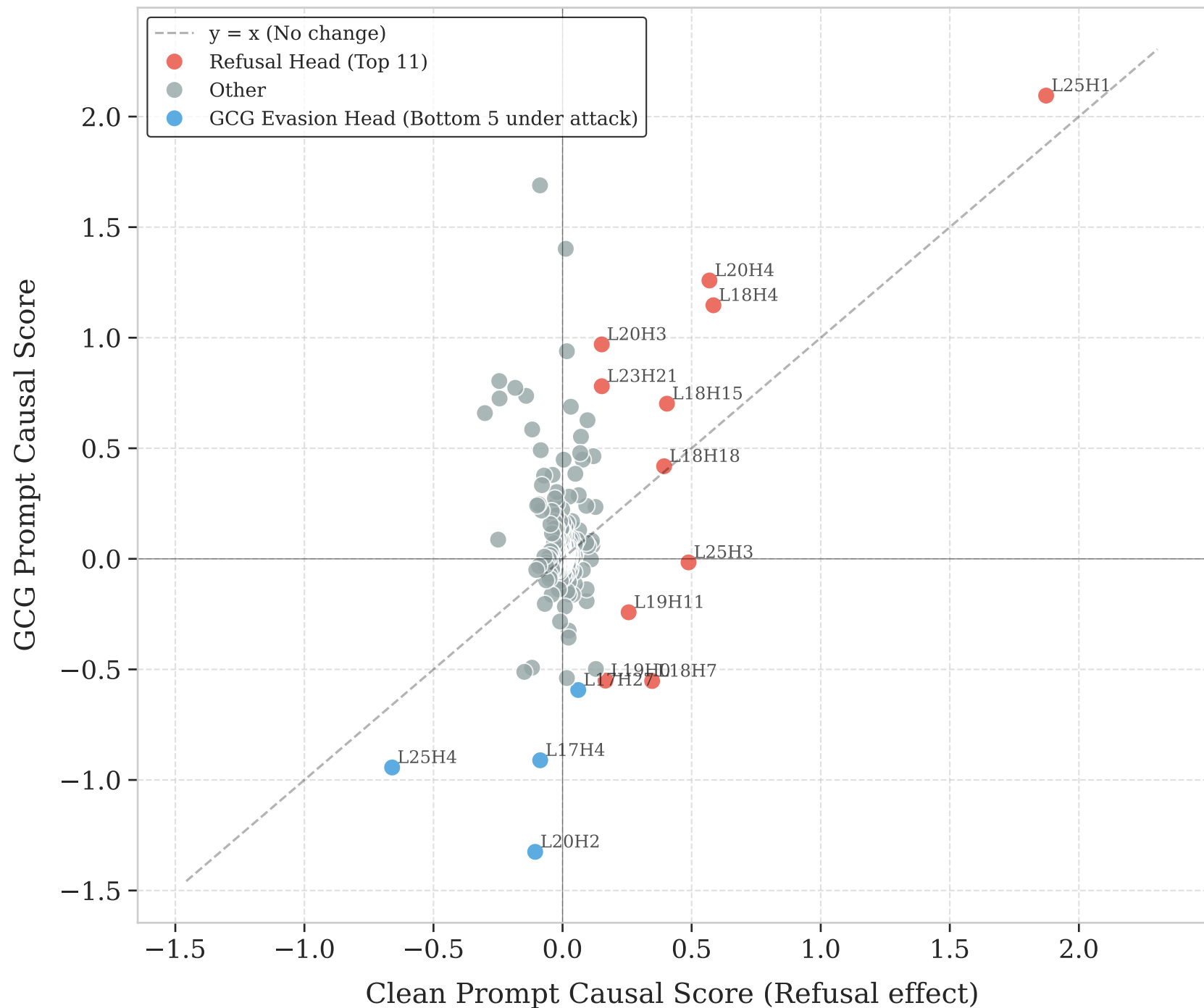
Activation Patching Scores: Clean vs. GCG Target
