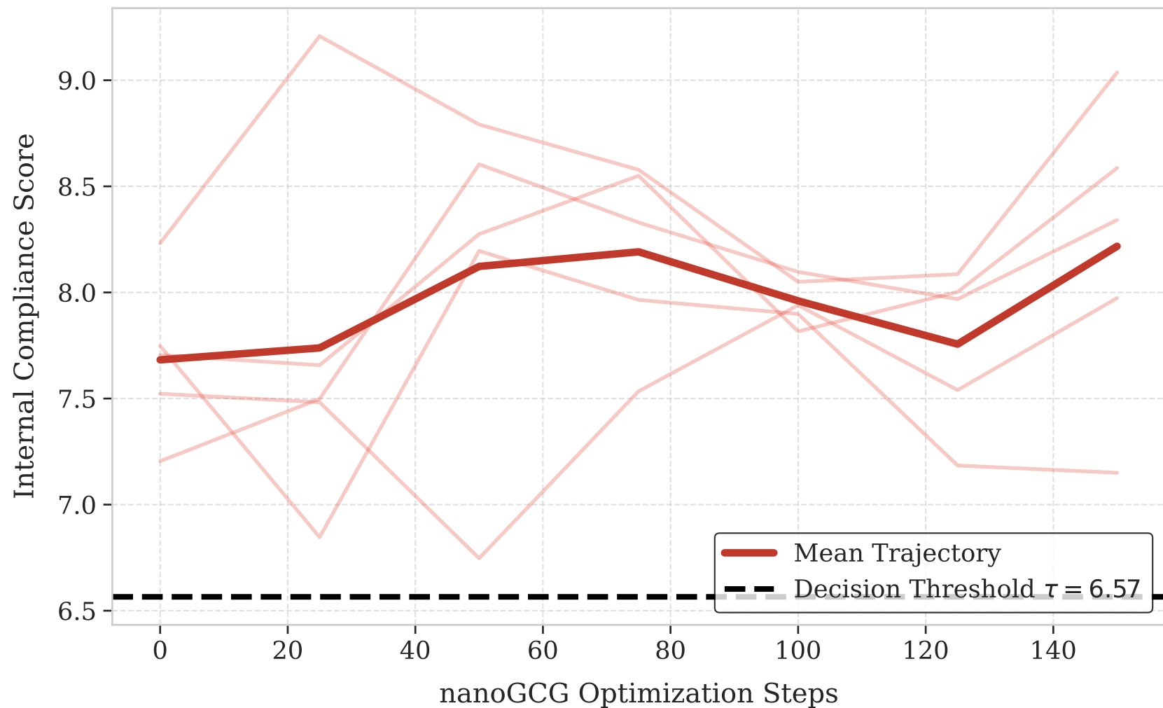
GCG Compliance Score Tracks Optimization Steps
