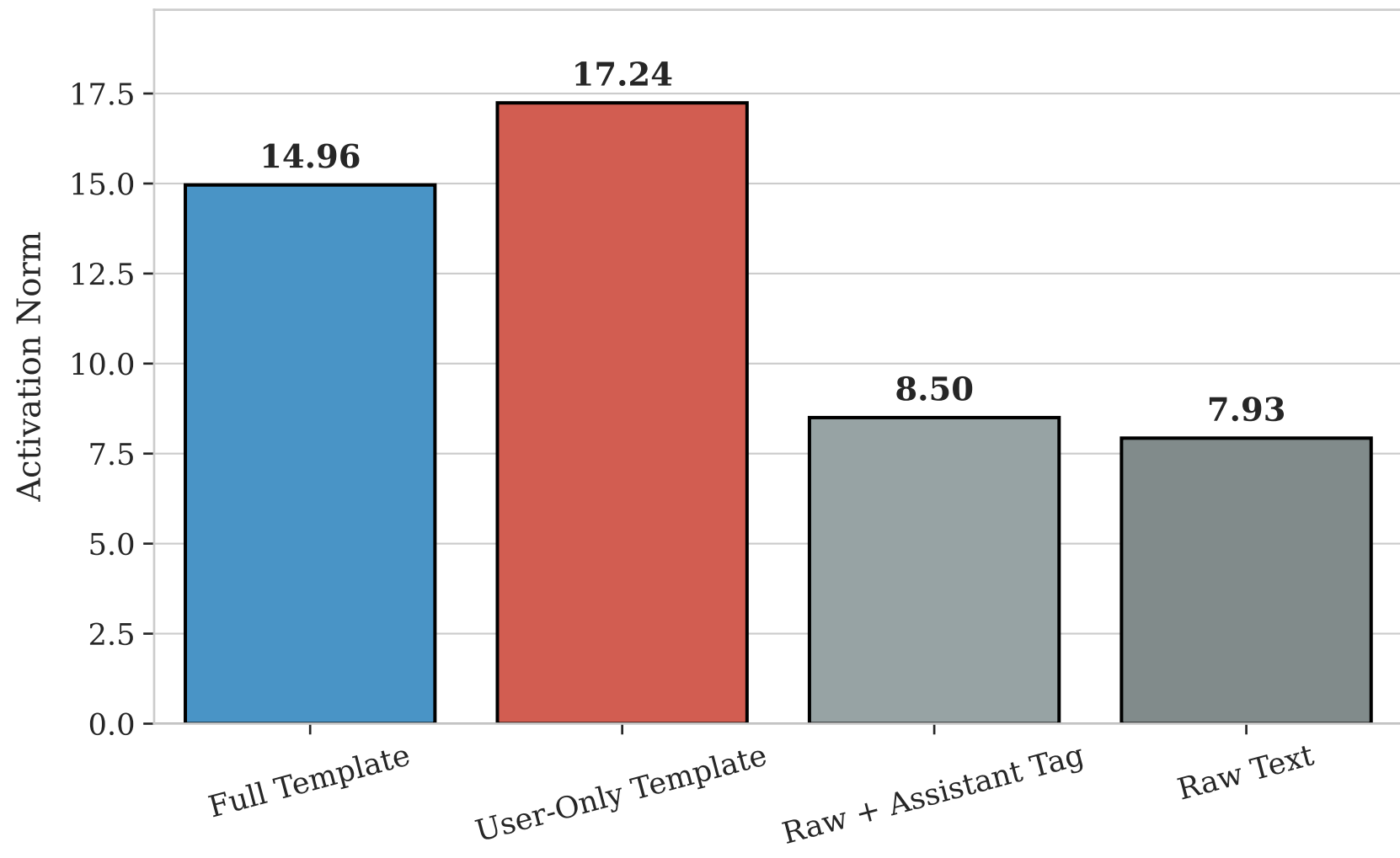
Activation Norm of L25-H1 (Refusal Target) Across Templates
