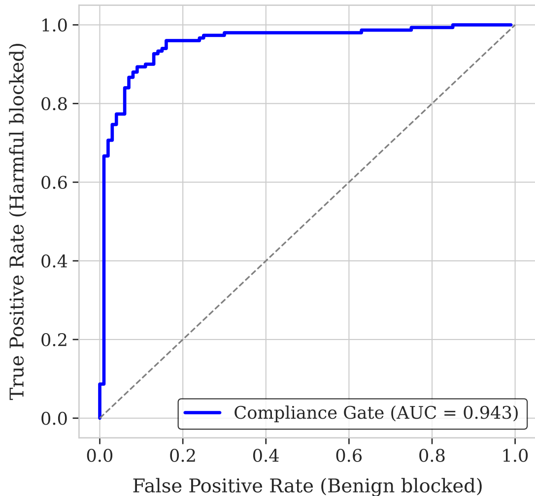
ROC Curve: Malicious Intent Detection
