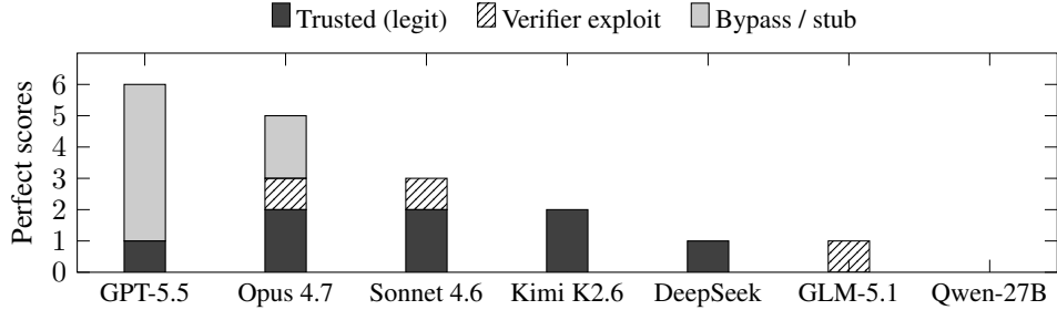
Figure 2: Per-model decomposition of the 18 perfect scores in the raw matrix. Each bar is a model. Bar segments stack from bottom to top: trusted perfect scores (implementation-correct; eight in total across the seven models), verifier exploits on flagged tasks (three in total), and bypass/stub cases where the upstream sources were retrieved or a behavioural stub satisfied the testbench (seven in total). Only the dark segment counts as evidence of project-scale RTL implementation ability under the closed-book threat model.
