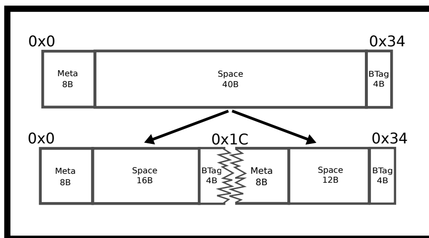
Figure 5.7: Malloc split
