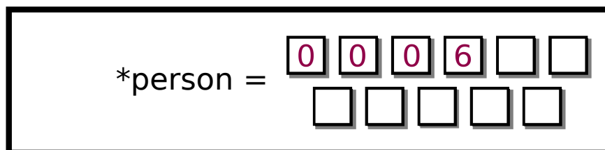
Figure 3.2: Struct pointing to 11 boxes, 4 filled with 0006, 7 empty
