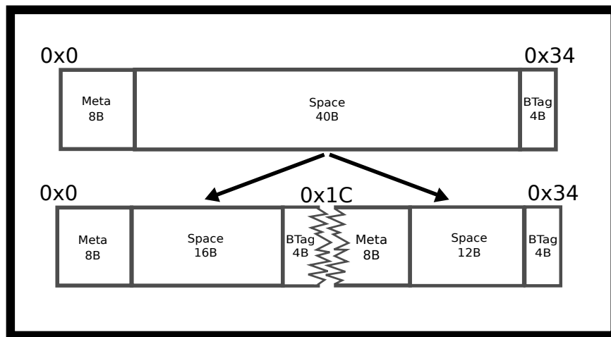
Figure 5.7: Malloc split
