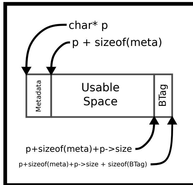
Figure 5.6: Malloc addition
