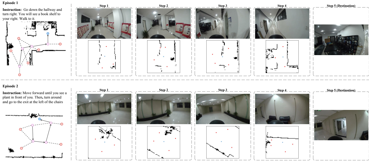
Figure 5: Qualitative results of two real-world navigation episodes using DIP 2 . For each episode, we visualize the instruction and the overall trajectory. At each navigation step, we present the front-facing observation and the predicted local waypoints.
