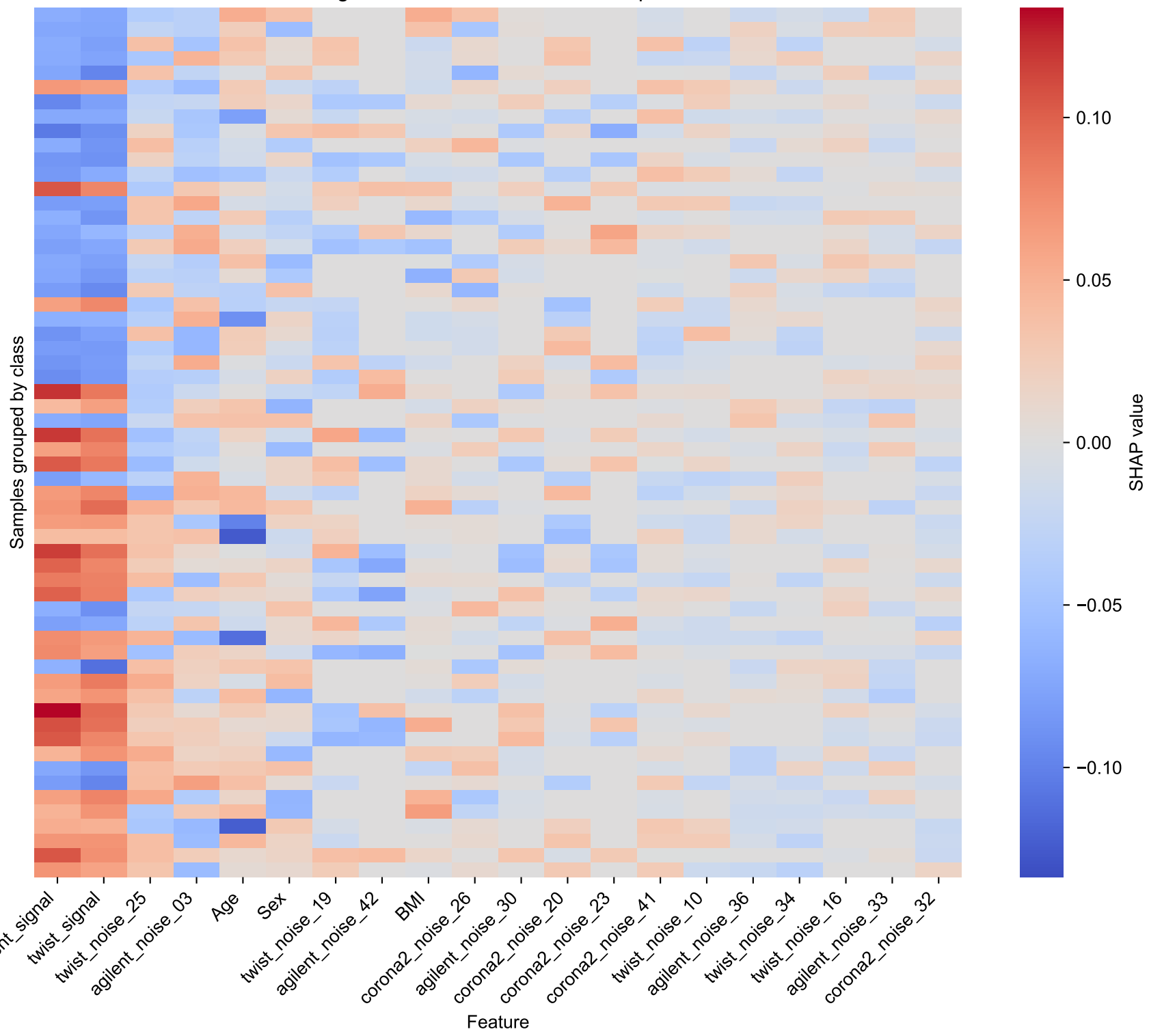
Signed SHAP values across samples
