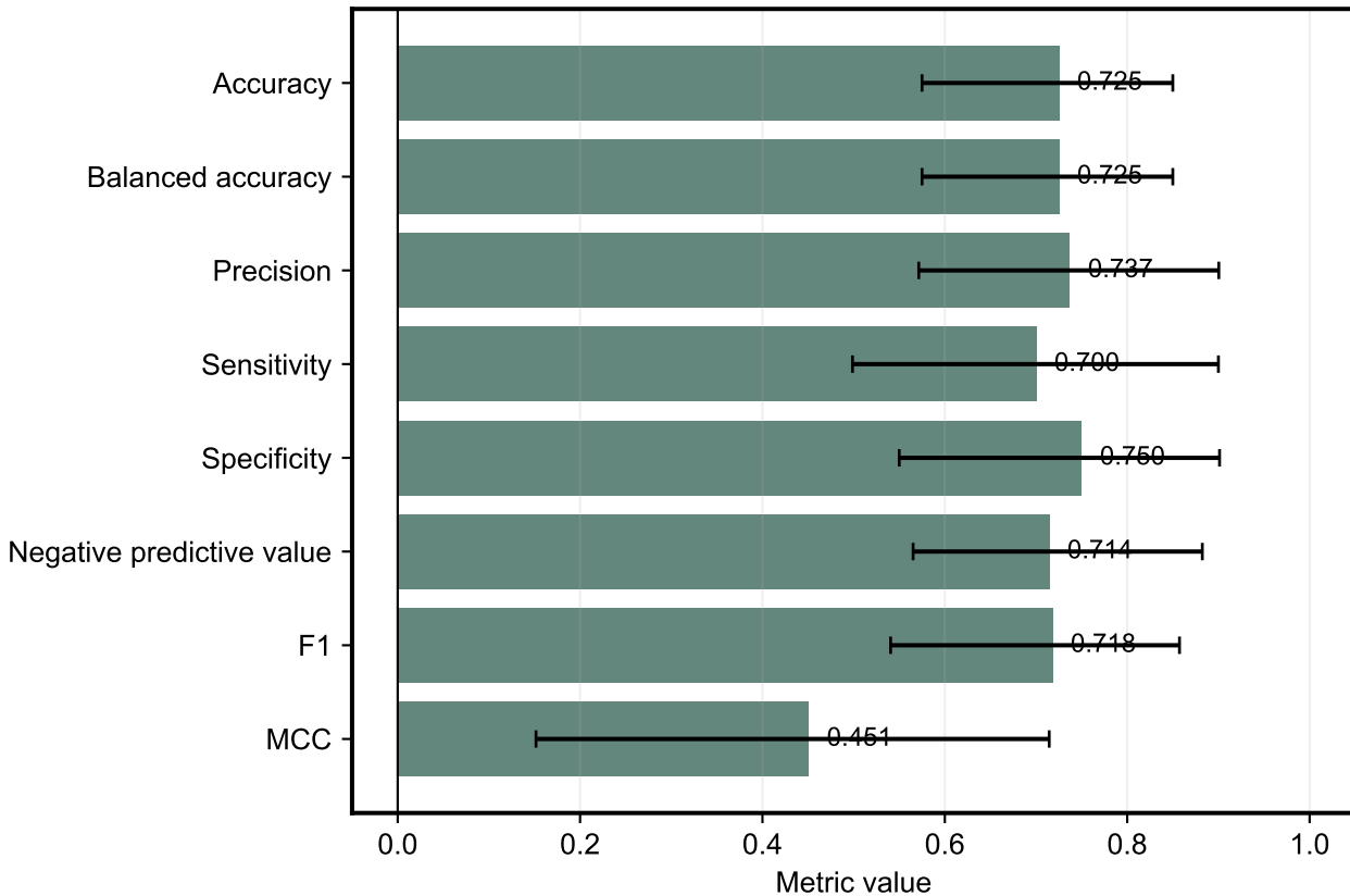
Threshold-dependent performance (threshold = 0.50) (95% stratified bootstrap interval (n=1000))
