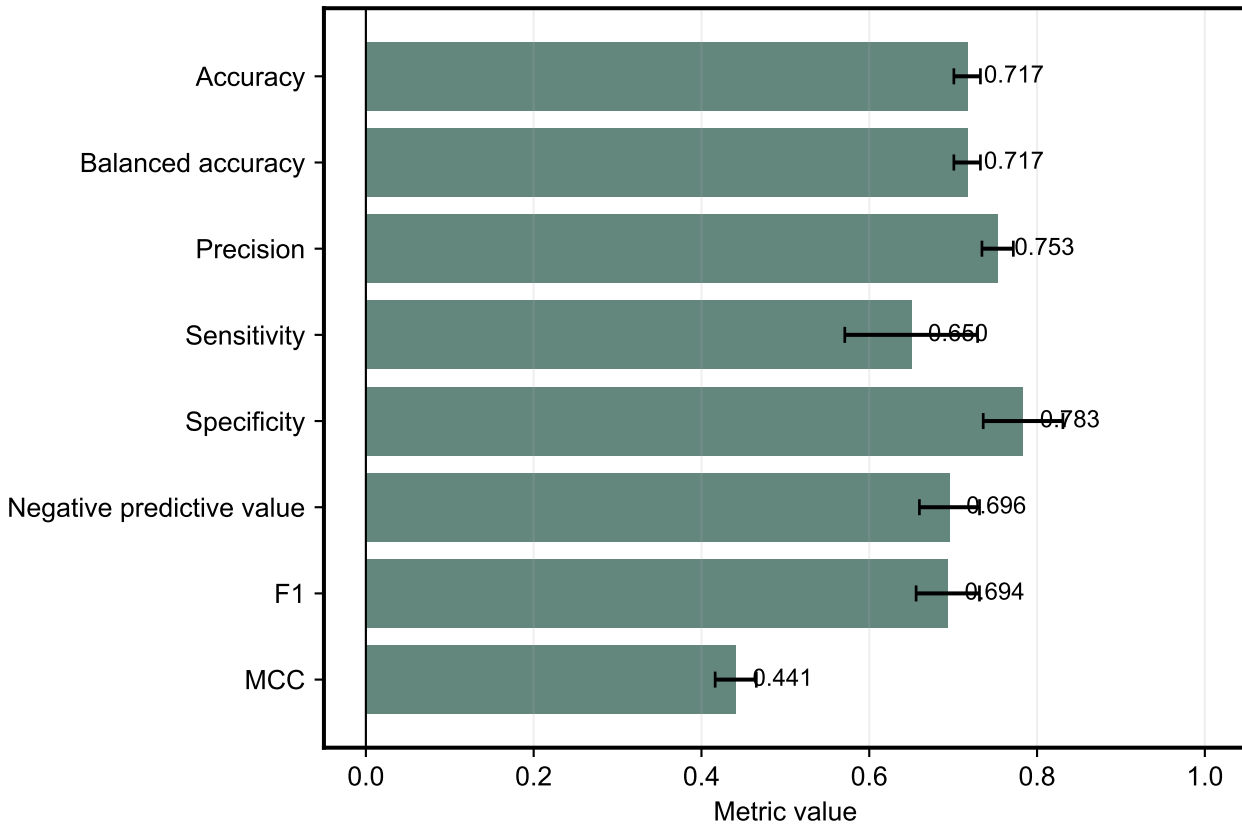
Threshold-dependent performance (threshold = 0.50) (2.5–97.5% empirical interval across 2 runs)
