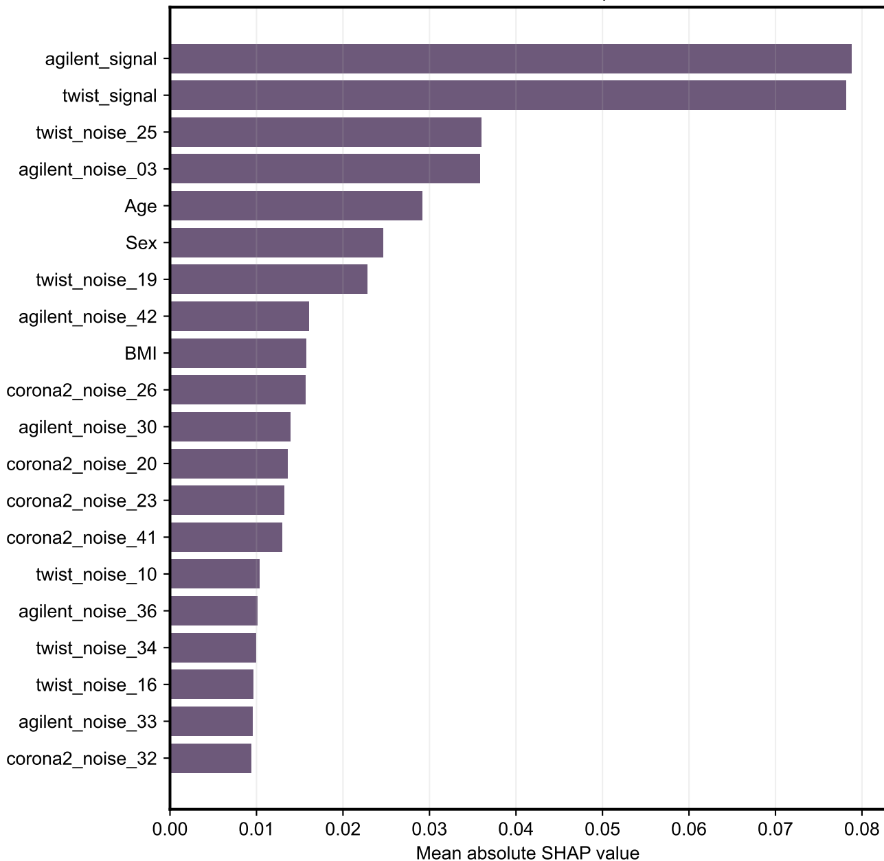
Global SHAP feature importance
