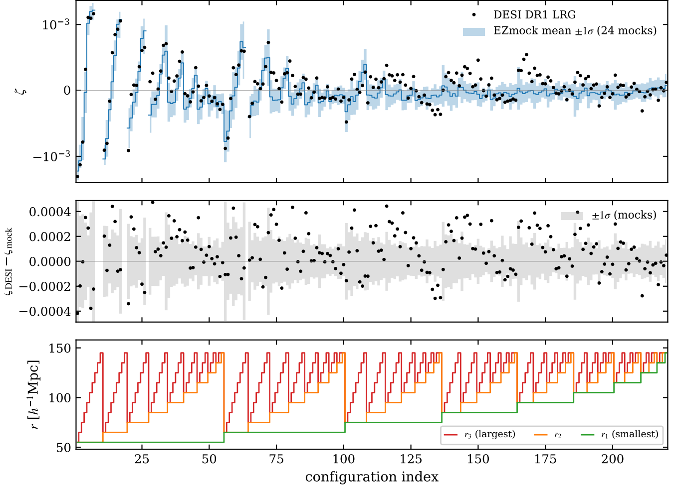
Figure 7. DESI DR1 LRG 3PCF versus the EZmock ensemble over all 220 triangle configurations ( 50 < r < 150 h^{-1} \text{Mpc} , 10 h^{-1} \text{Mpc} bins; NGC, SGC, and both redshift bins combined at the count level in data and mocks). Top: \zeta (symlog axis), DESI points over the mock mean \pm 1\sigma band (24 realisations). Middle: the residual \zeta_{\text{DESI}} - \bar{\zeta}_{\text{mock}} with the \pm 1\sigma mock band. Bottom: a key to the configuration axis — the three sorted triangle side-length bins r_1 \leq r_2 \leq r_3 of each configuration, so a vertical read-off gives the triangle shape. The nested staircase reflects the lexicographic ordering of the canonical configurations.
