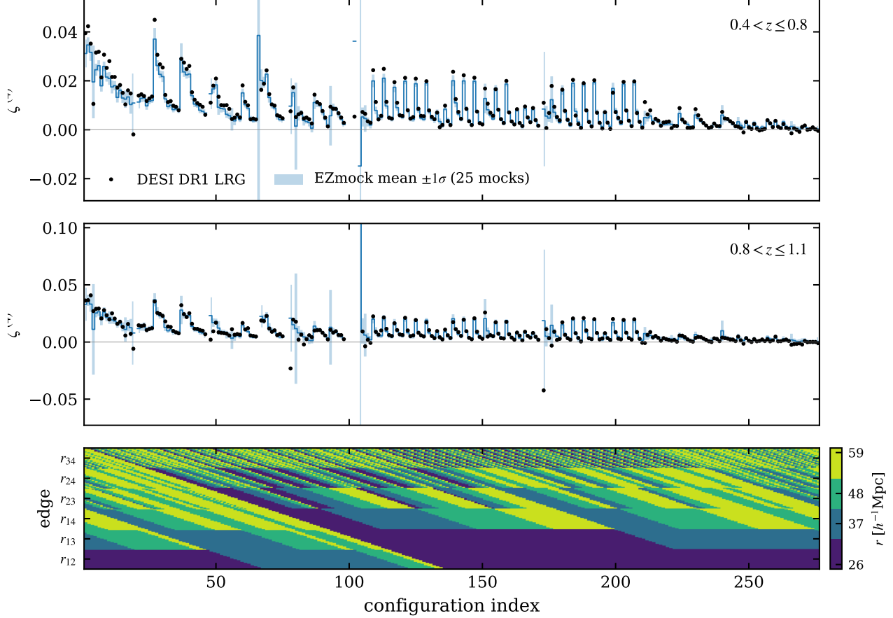
Figure 8. DESI DR1 LRG 4PCF ( \zeta^{(4)} = \text{NNNN}/\text{RRRR} ) versus the EZmock ensemble over all 276 configurations ( 20 < r < 65 h^{-1}\text{Mpc} , 4 radial bins; canonical configuration ordering), for the two redshift bins (top, middle). NGC and SGC are combined at the count level in both data and mocks; the band is the ensemble mean \pm 1\sigma over 25 realisations. Isolated wide bands mark sparse configurations with poorly determined mock scatter. The bottom panel is a key to the configuration axis: each tetrahedron is specified by the bins of its six pairwise edges ( r_{12}, r_{13}, r_{14}, r_{23}, r_{24}, r_{34} ), shown here as the bin-centre scale (colour) of each edge for every configuration, so a vertical stripe recovers the physical scales of any configuration. The diagonal block structure reflects the lexicographic ordering of the canonical 6-tuples.
