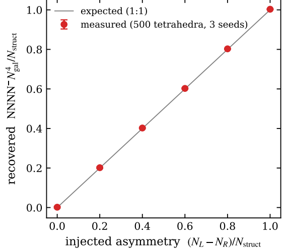
Figure 6. Signal-injection test of the parity-odd 4PCF. Catalogues of 500 isolated chiral tetrahedra with left-handed fraction x are measured with the GPU parity kernel; the count-normalised odd channel at the injected configuration recovers the injected asymmetry 2x - 1 (grey 1:1 line) to 0.3%, with the balanced case consistent with zero. Error bars show the scatter over three random realisations.
