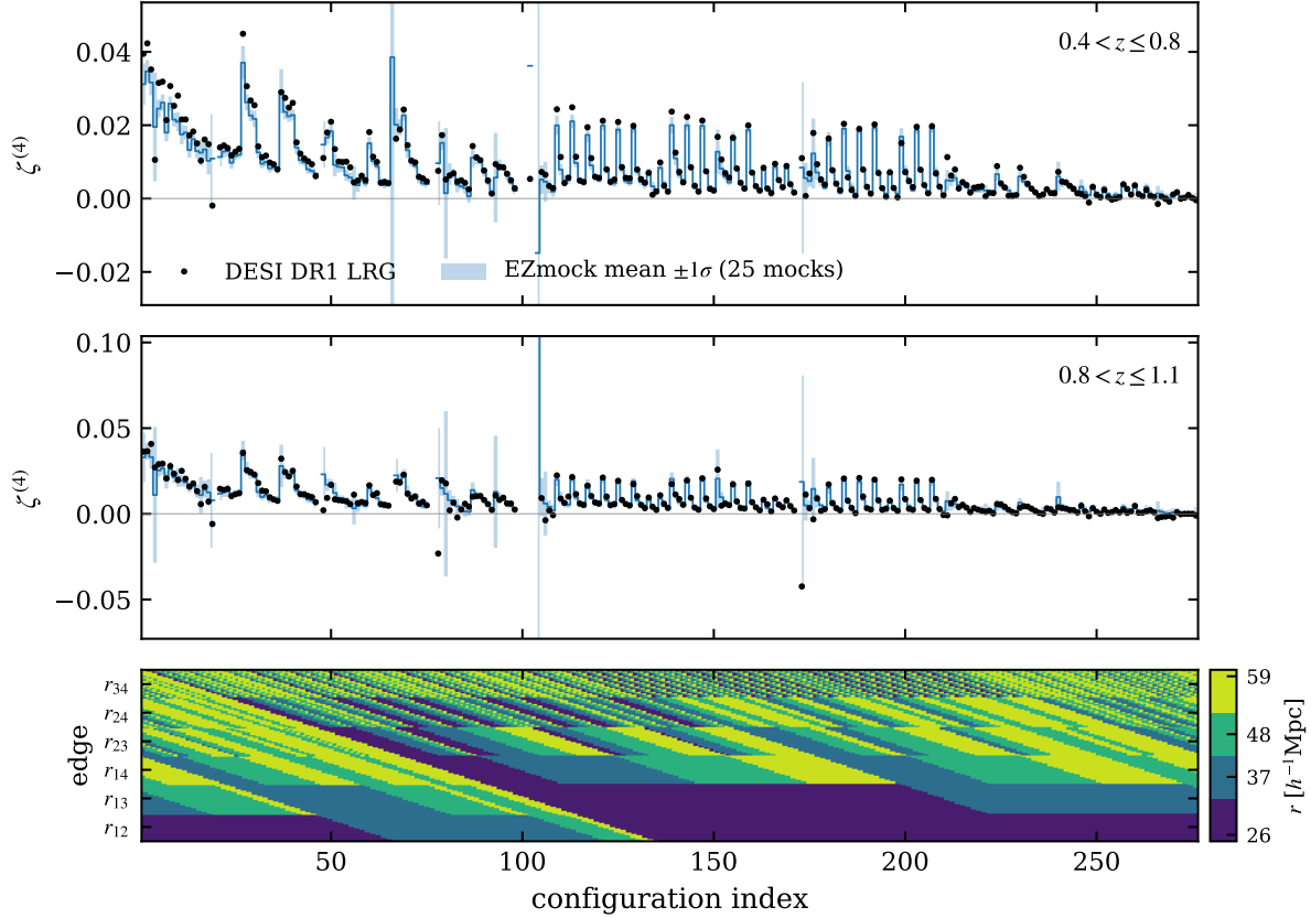
Figure 8. DESI DR1 LRG 4PCF ( \zeta^{(4)} = \text{NNNN}/\text{RRRR} ) versus the EZmock ensemble over all 276 configurations ( 20 < r < 65 h^{-1} \text{Mpc} , 4 radial bins; canonical configuration ordering), for the two redshift bins (top, middle). NGC and SGC are combined at the count level in both data and mocks; the band is the ensemble mean \pm 1\sigma over 25 realisations. Isolated wide bands mark sparse configurations with poorly determined mock scatter. The bottom panel is a key to the configuration axis: each tetrahedron is specified by the bins of its six pairwise edges ( r_{12}, r_{13}, r_{14}, r_{23}, r_{24}, r_{34} ), shown here as the bin-centre scale (colour) of each edge for every configuration, so a vertical stripe recovers the physical scales of any configuration. The diagonal block structure reflects the lexicographic ordering of the canonical 6-tuples.
