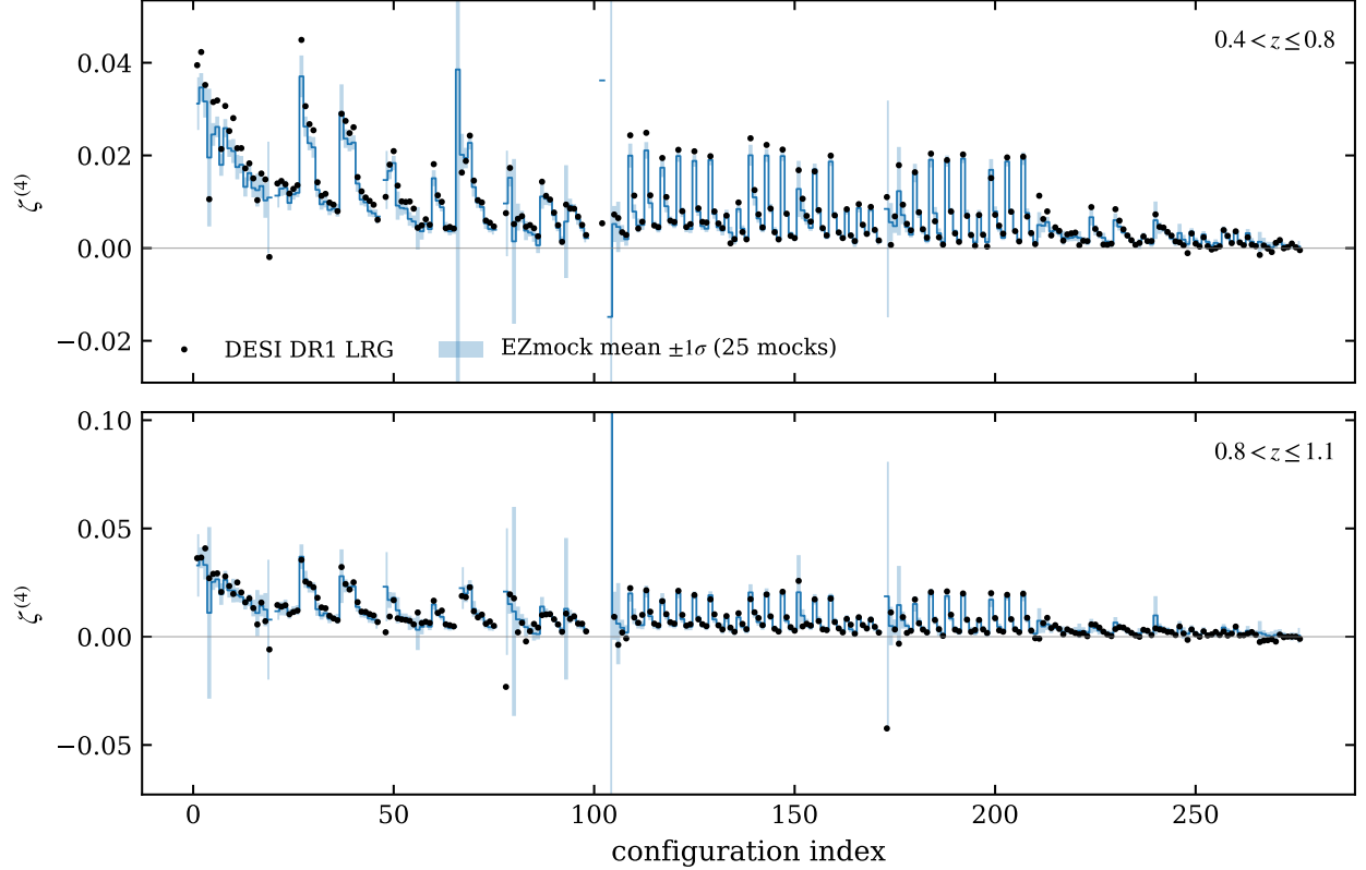
Figure 8. DESI DR1 LRG 4PCF ( \zeta^{(4)} = \text{NNNN/RRRR} ) versus the EZmock ensemble over all 276 configurations ( 20 < r < 65 h^{-1}\text{Mpc} , 4 radial bins; canonical configuration ordering), for the two redshift bins. NGC and SGC are combined at the count level in both data and mocks; the band is the ensemble mean \pm 1\sigma over 25 realisations. Isolated wide bands mark sparse configurations with poorly determined mock scatter.
