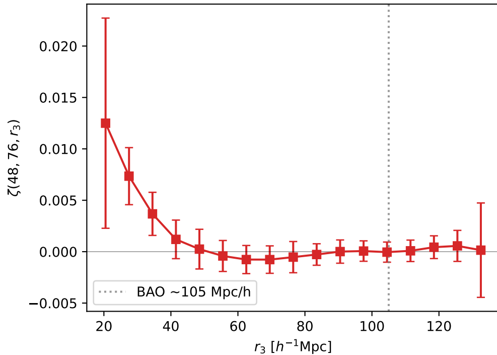
isoceles slice (48, 76, r_3 )
