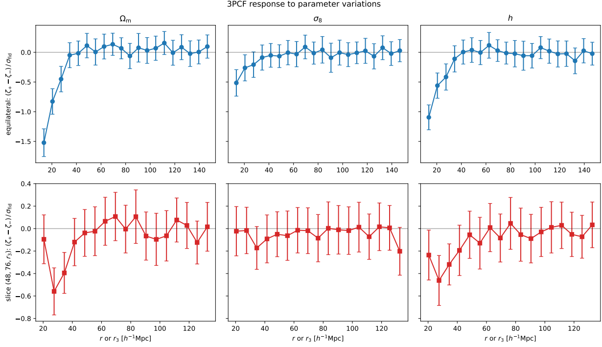
Figure 8. Response of the 3PCF to the Quijote parameter variations, in units of the single-realisation fiducial scatter, for the equilateral cut (top row) and the isocles slice \zeta(48, 76, r_3) (bottom row). Error bars propagate the ensemble errors of the variation means (50 realisations per side). The responses are confined to quasi-linear scales with the same parameter hierarchy in both cuts, and the matched number density suppresses the \sigma_8 response relative to the shape parameters \Omega_m and h (see text).
